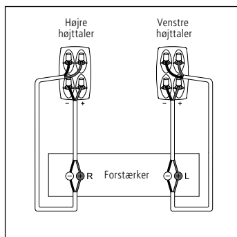
Bi-wiring
