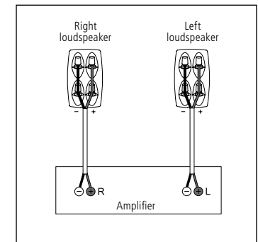
Normal wiring
