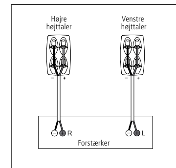
Normal kabling
